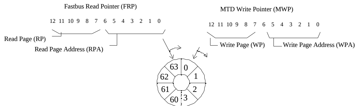
Figure 5-2 1881M Circular Buffer
