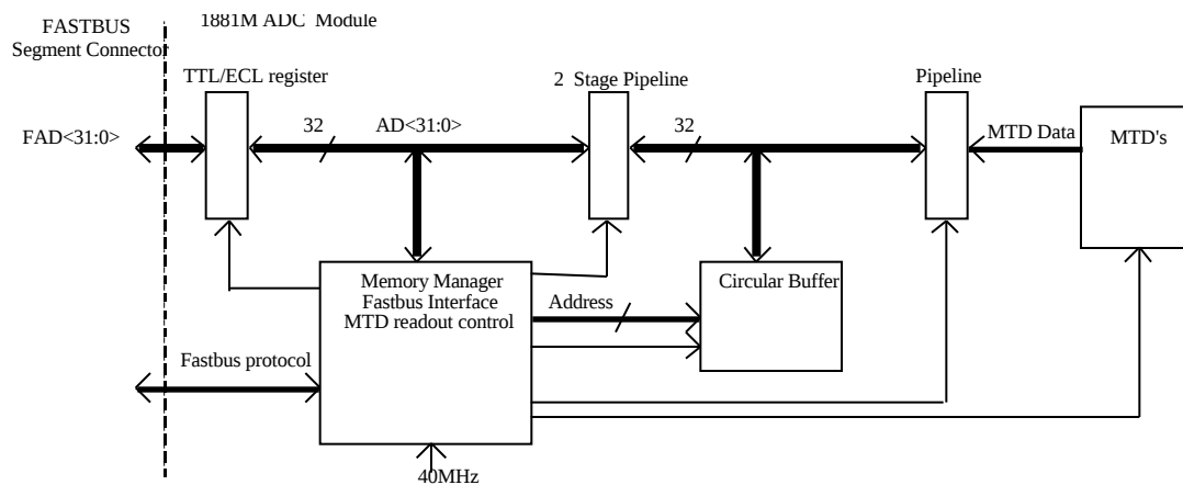
Figure 5-1 Simplified 1881M Interface/Buffer Block Diagram
