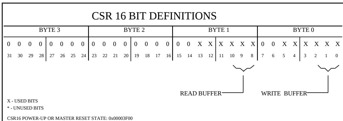
Figure 2-4 CSR16 Bit Definition
