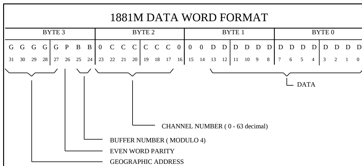
Figure 2-6 1881M Data Word
