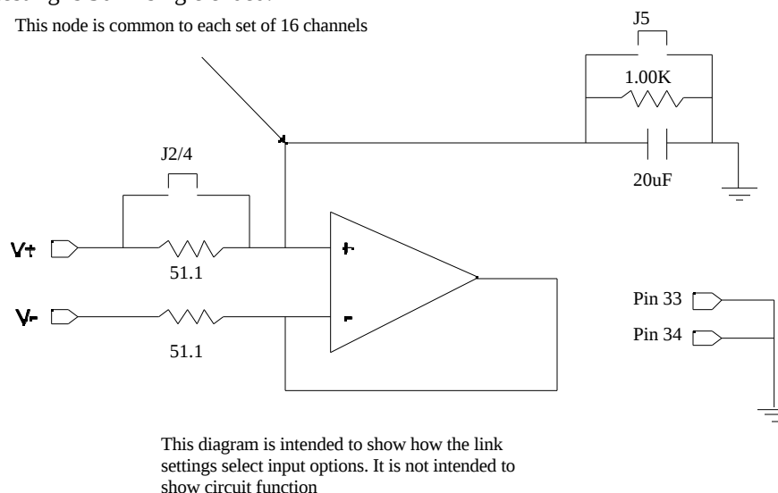
Figure 3-1 Input Circuit
