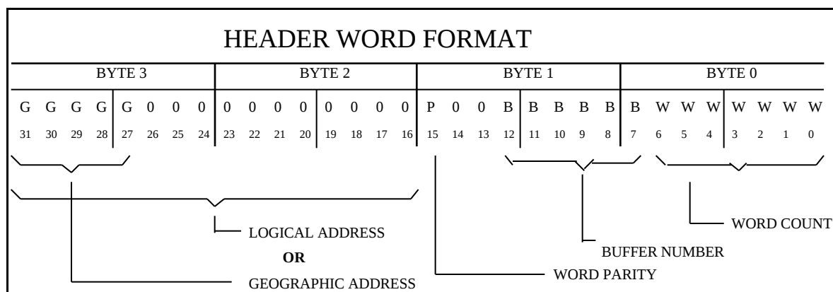
Figure 2-5 1881M Header Word
