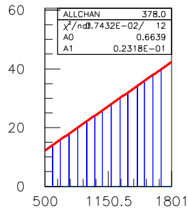
TDC.1290.sl.10.ch.01
