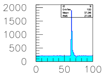
FADC SPECTRA
