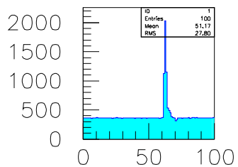
FADC SPECTRA
