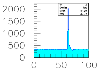
FADC SPECTRA
