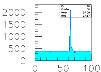
FADC SPECTRA
