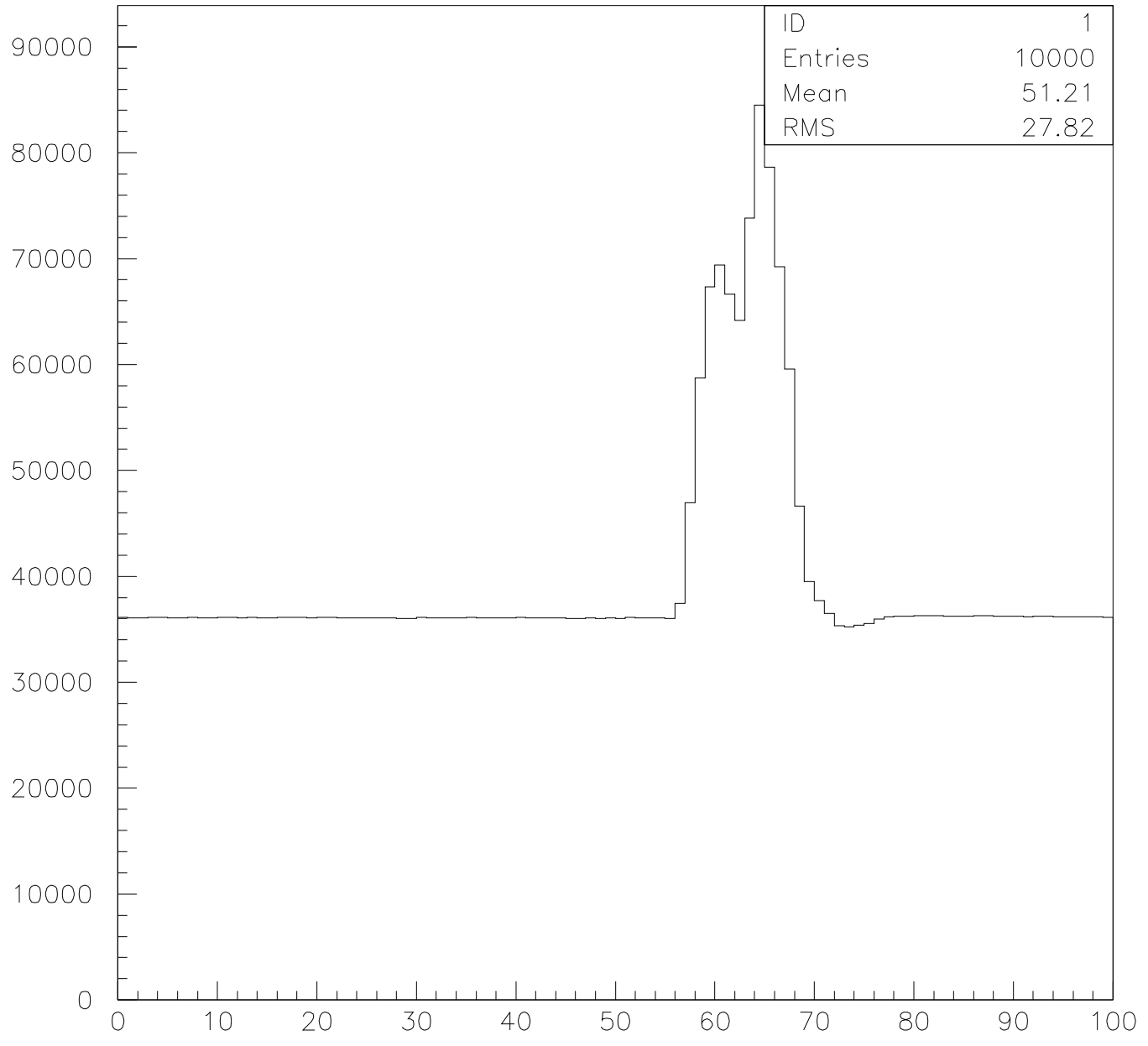
FADC SPECTRA
