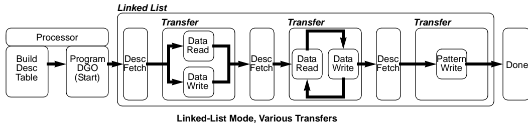
Figure 19: Linked-list Mode
