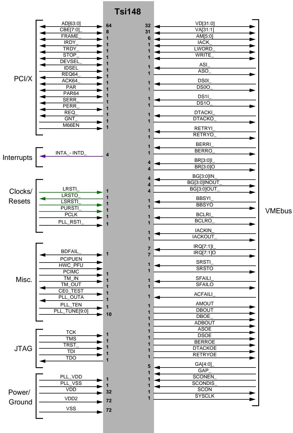
Figure 33: Signal Grouping
